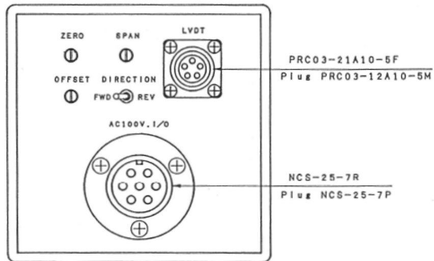
Back panel
